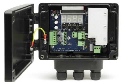
Leak Alert 73 with lid open showing 3 LEDs, display and internal set up keys
